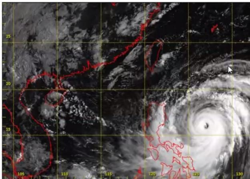
Super Typhoon Mangkhut (超強颱風山竹) 11:30 p.m. 13 September 2018
